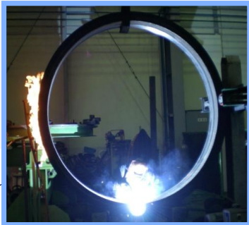
Weld Overlay
